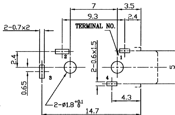
PC BOARD HOLE LAYOUT (Tols:±0.1) (VIEW FROM DIRECTION OF INSERTION TO PCB)
