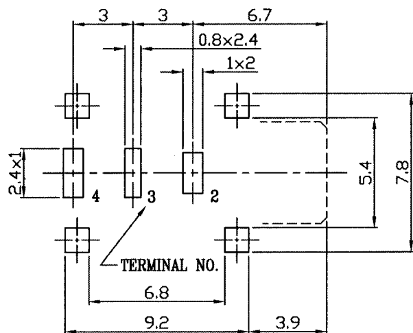
PC BOARD HOLE LAYOUT(GEN TOLS: \pm 0.1 )
