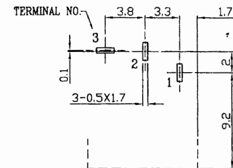
PC BOARD HOLE LAYOUT (TOLS: ±0.1) (VIEW FROM INSERTION TO PCB)
