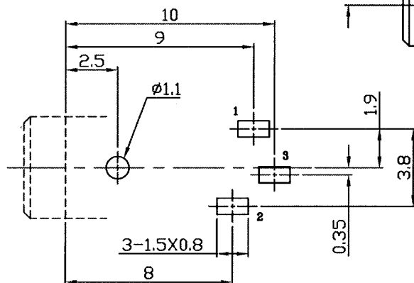
PC BOARD HOLE LAYOUT (BOTTOM VIEW) TOLS : ±0.1
