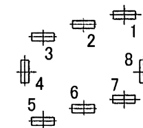
TERMINAL POSITION (BOTTOM VIEW)
