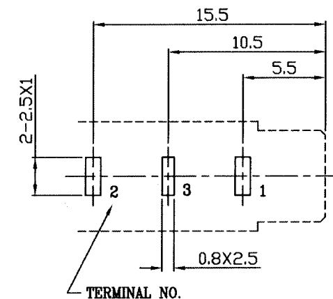
PC BOARD HOLE LAYOUT
