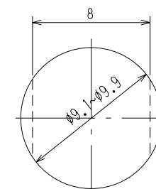
取付板板厚 Thickness of mounting board t=1.0\sim 1.8
