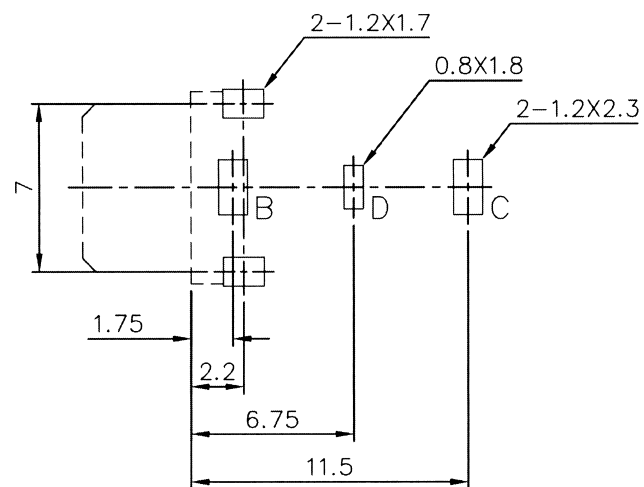
HOLE LAYOUT (BOTTOM VIEW)
