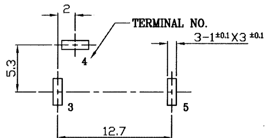
PC BOARD HOLE LAYOUT (GEN TOLS: ±0.2) (UPPER VIEW FROM THE DIRECTION OF INSERTION TO PCB.)
