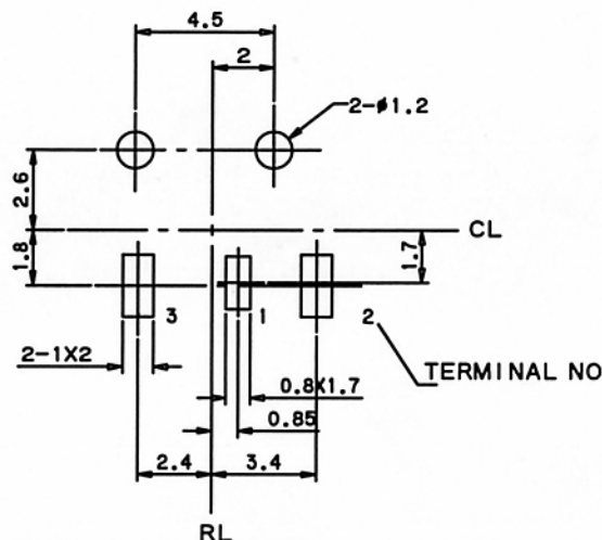
PC BOARD HOLE LAYOUT TOLS : ±0.1 (VIEW FROM DIRECTION OF INSERTION TO PCB)
