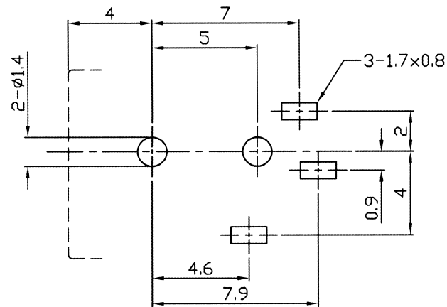
PC BOARD HOLE LAYOUT (UPPER VIEW FROM DIRECTION OF INSERTION TO PCB)
