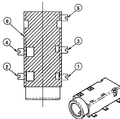
プラグ～ジャック接点互換図 Interchangeable drawing of contact point of plug-jack
