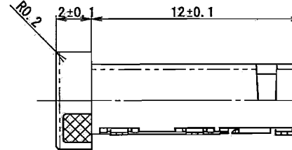
平坦度寸法規定 The degree size regulation of flat
