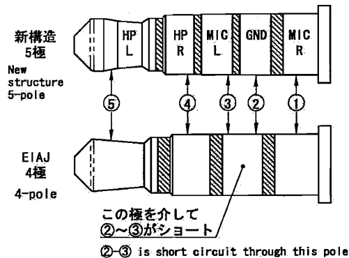
プラグ～ジャック接点互換図 Interchangeable drawing of contact point of plug-jack
